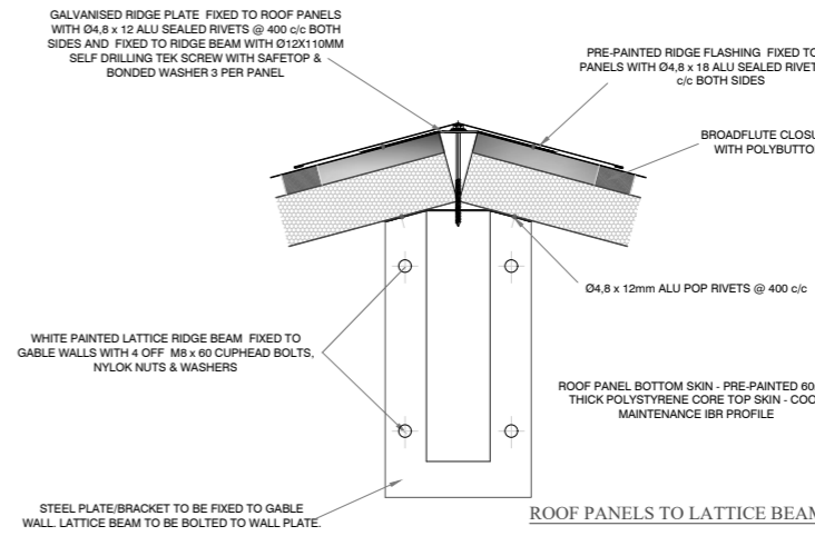
ROOF PANELS TO LATTICE BEAM DETAIL
