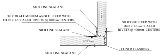
WALL TO WALL OUTSIDE CORNER FIXING DETAIL:
