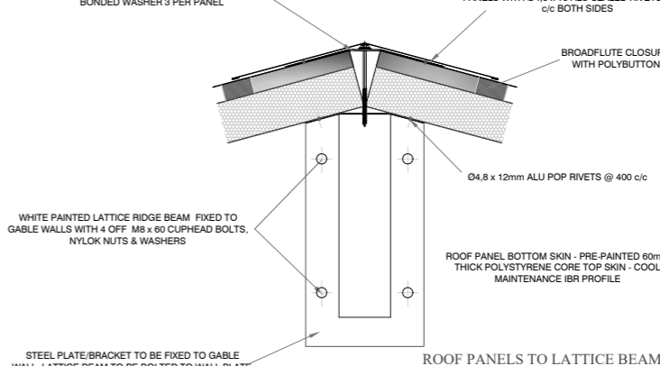
ROOF PANELS TO LATTICE BEAM DETAIL
