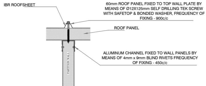
INTERNAL PARTITION WALL TO ROOF FIXING DETAIL
