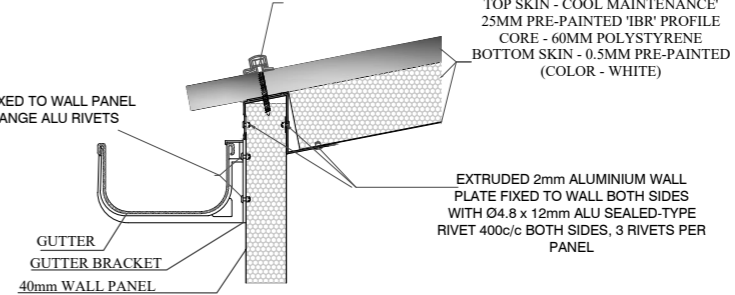
ROOF TO GUTTER DETAIL:
