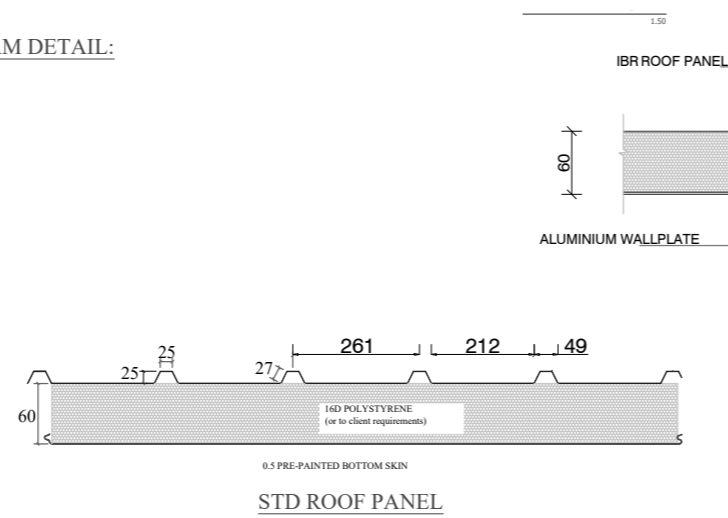
THICKNESS OF FIRE RETARDANT POLYSTYRENE CORE 40mm - 50mm (16D) VARIES 50mm - 200mm (16D)
