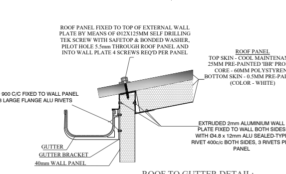
ROOF TO GUTTER DETAIL:
